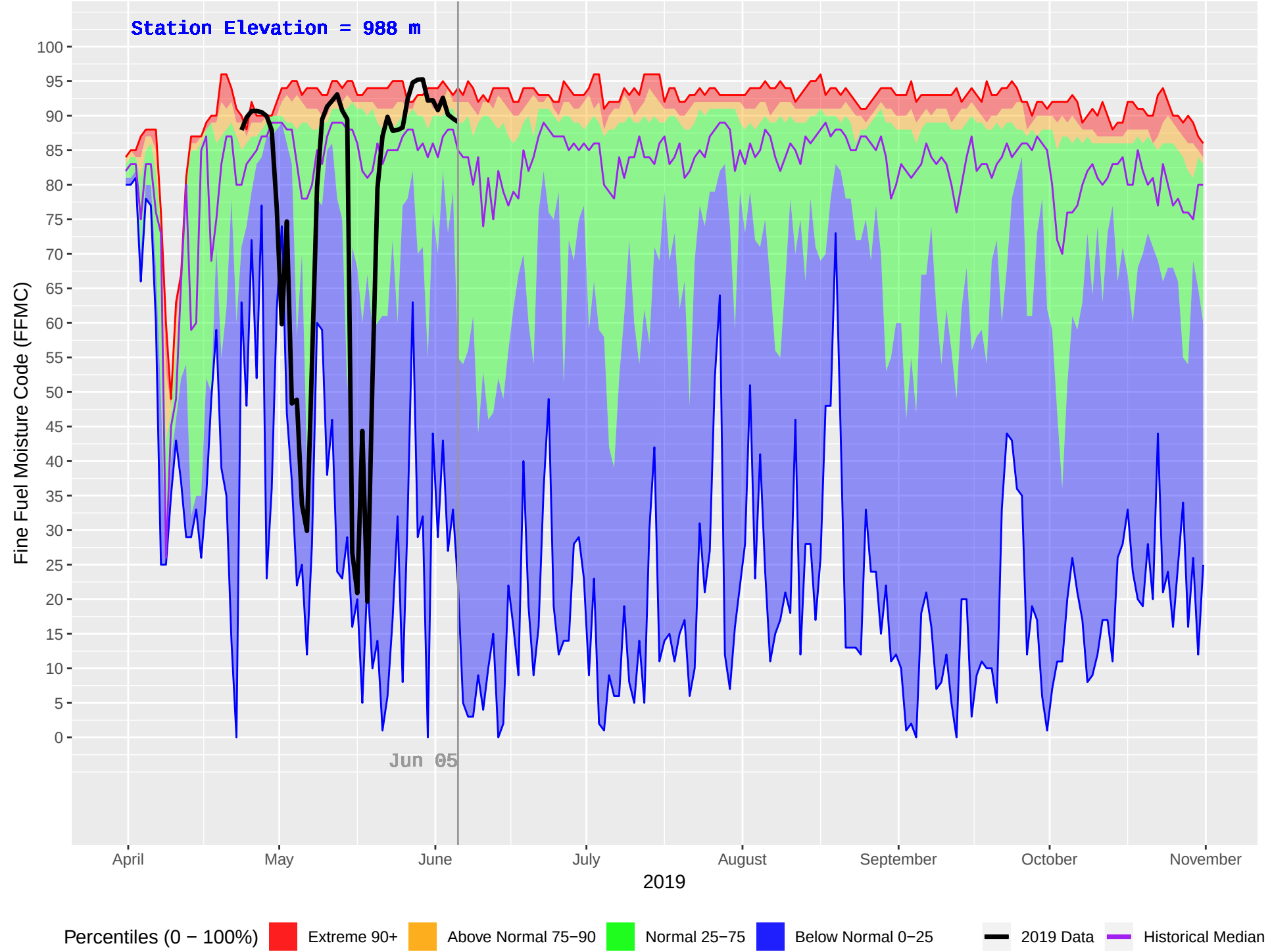
NOEL (437) : Historical (1993–2018) and Current (2019) Daily Fine Fuel Moisture Code (FFMC)
