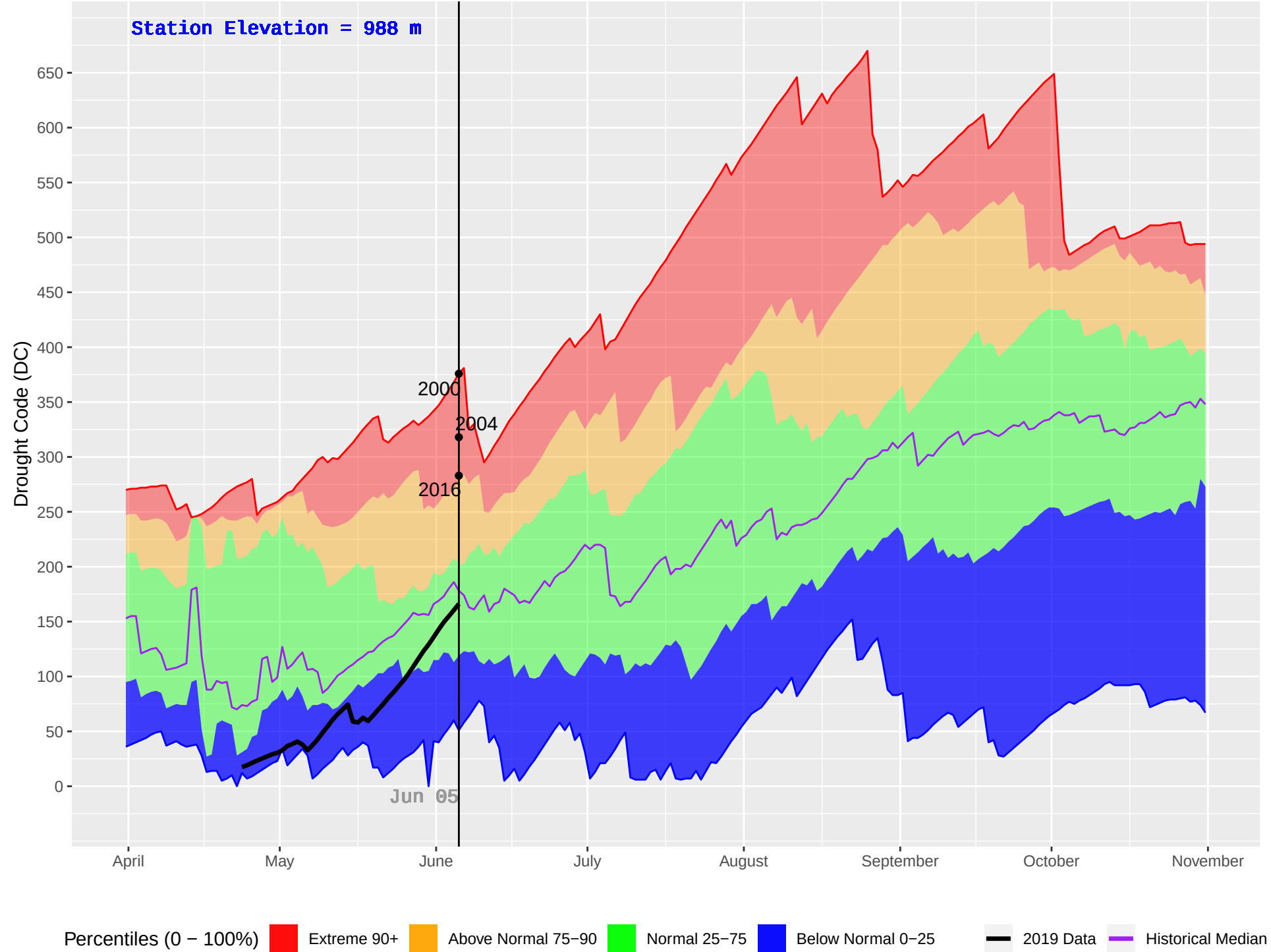
NOEL (437) : Historical (1993–2018) and Current (2019) Daily Drought Code (DC)
