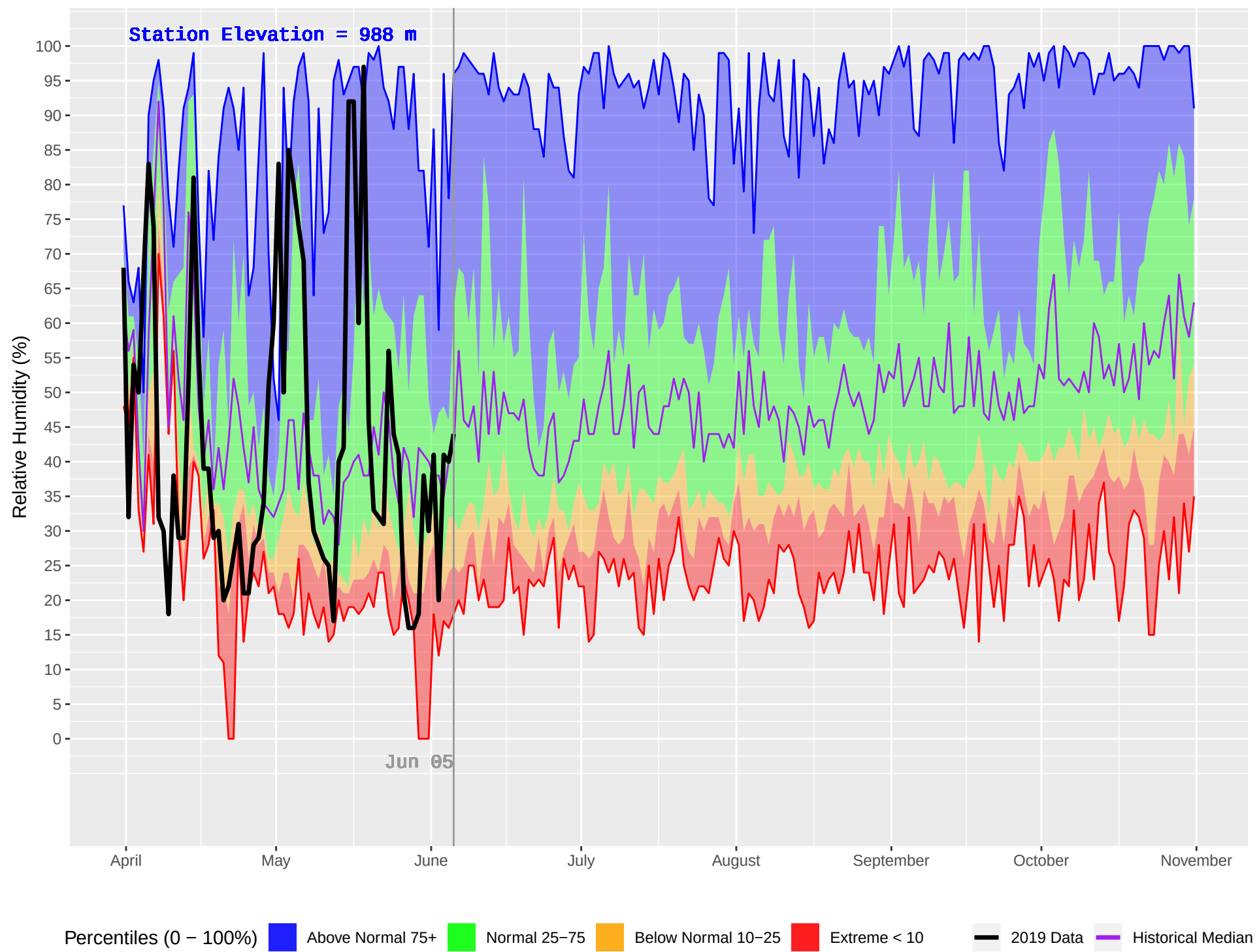
NOEL (437) : Historical (1993–2018) and Current (2019) Daily Relative Humidity
