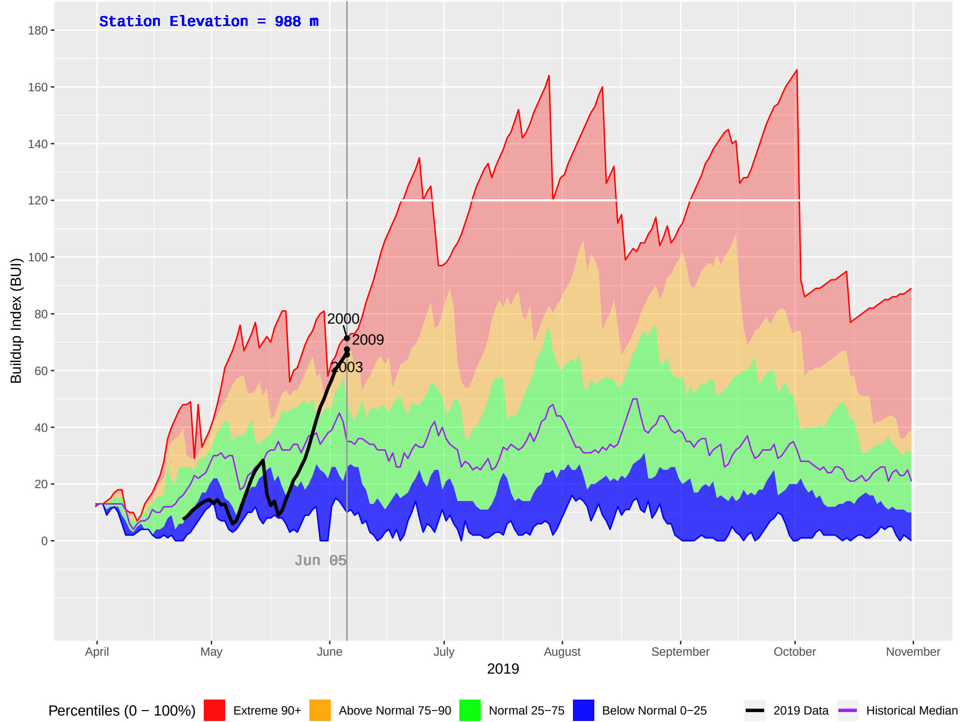
NOEL (437) : Historical (1993–2018), Current (2019) Daily Buildup Index (BUI)
