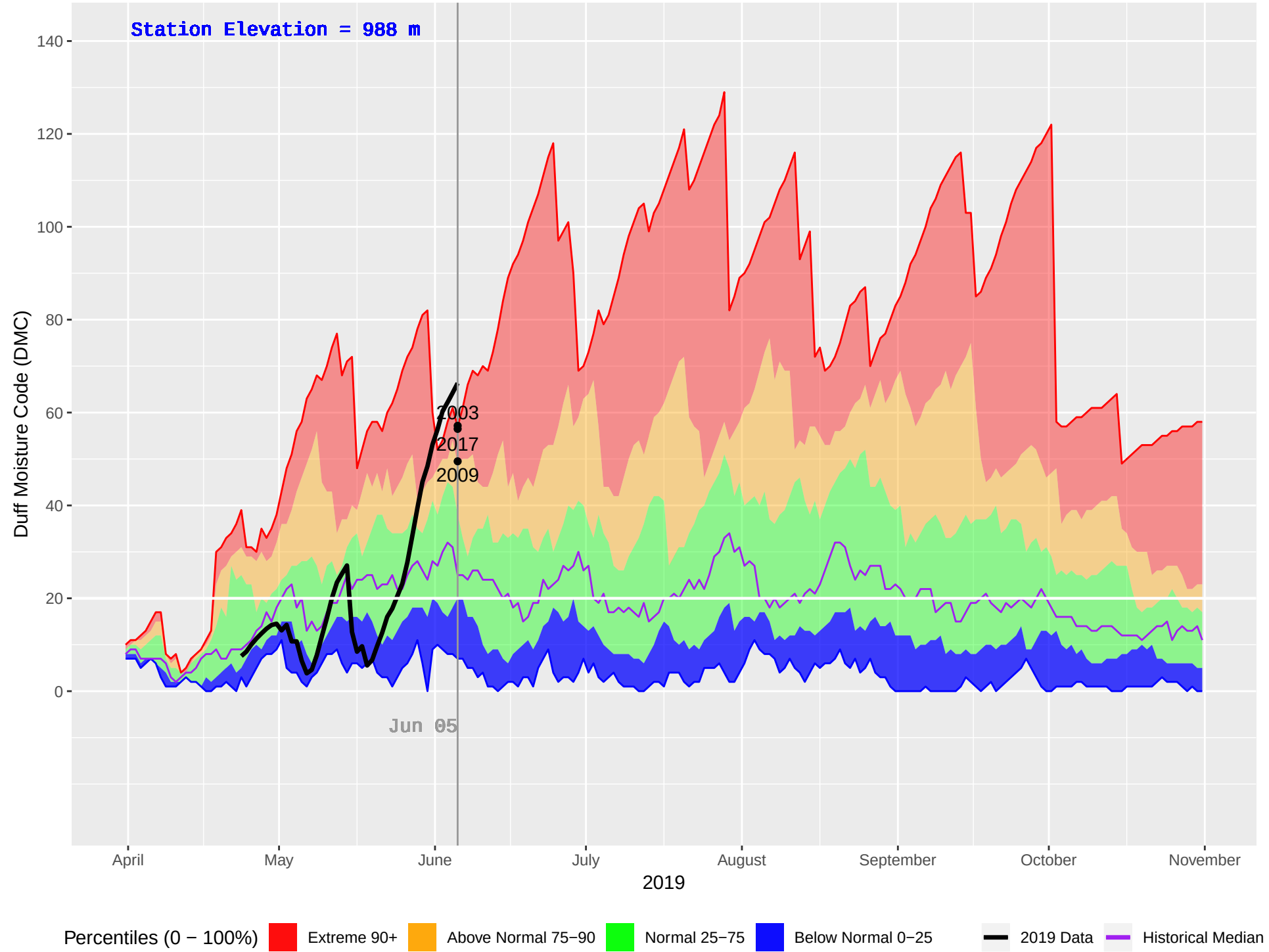
NOEL (437) : Historical (1993–2018), Current (2019) Daily Duff Moisture Code (DMC)
