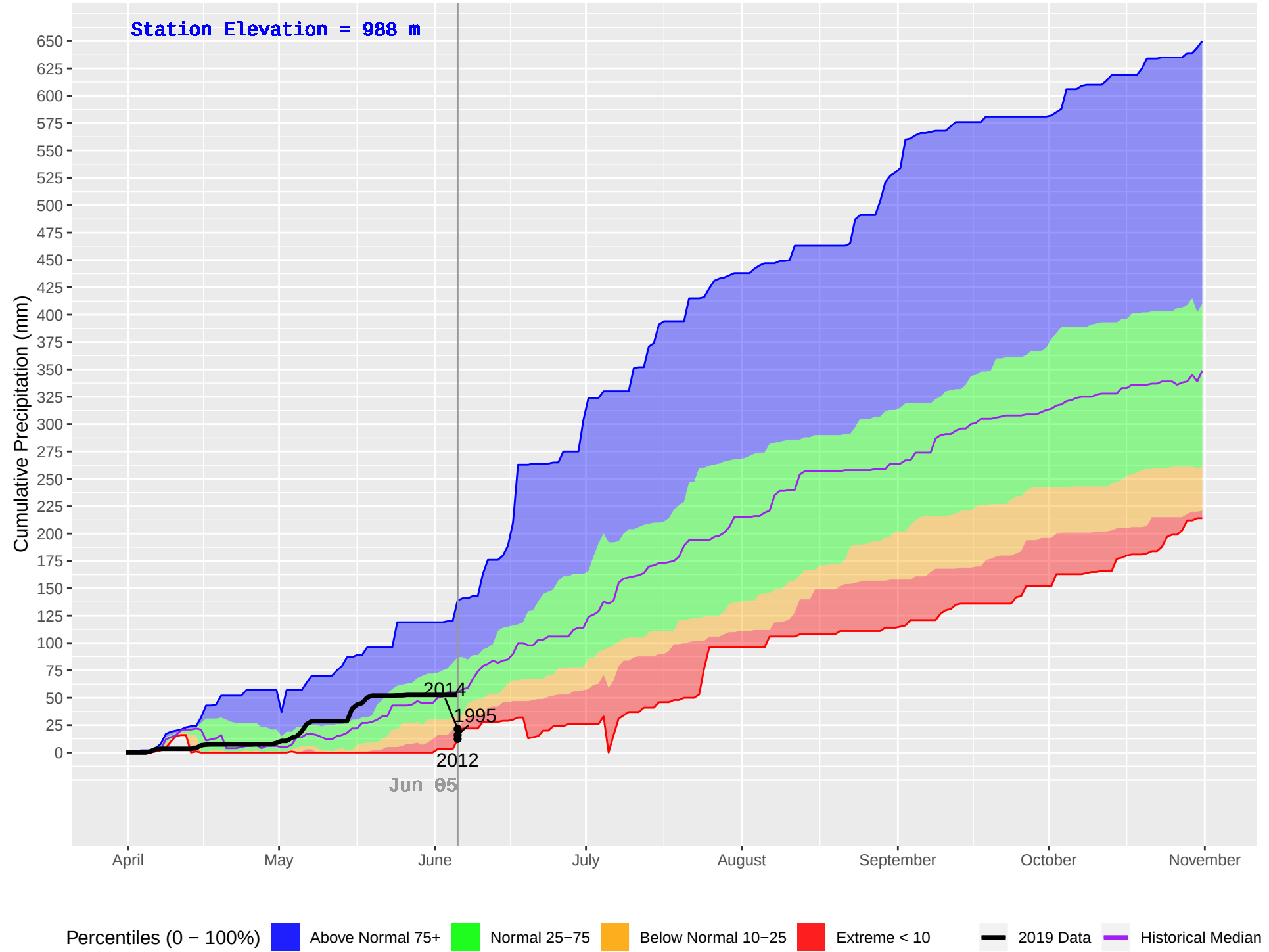
NOEL (437) : Historical (1993–2018), Current (2019) Daily Cumulative Precipitation
